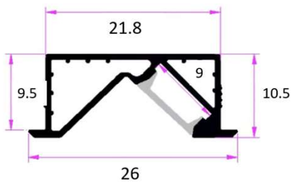
Angled Profile Joinery
